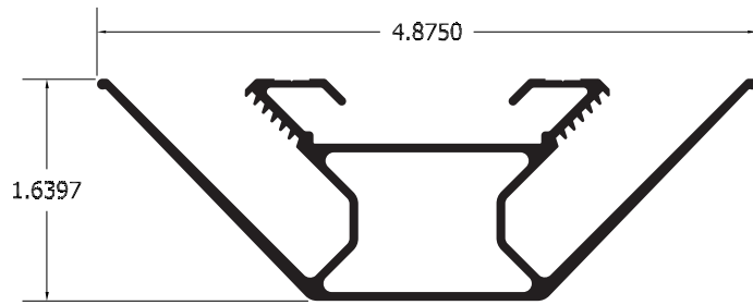
FLAT BLEED DOUBLE FACE TENSION BODY PART# 2230
